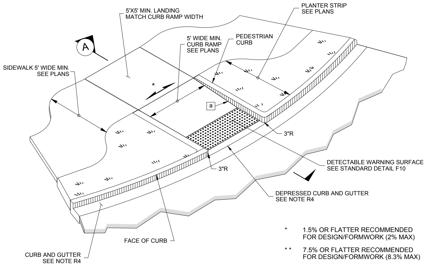
ISOMETRIC VIEW
