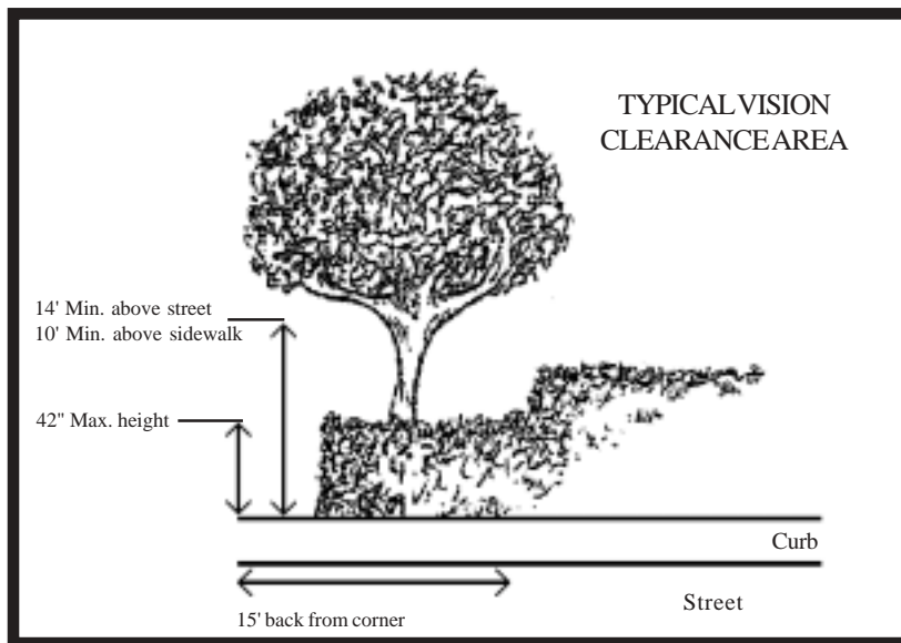
Figure 18.17.030-2 Vision Clearance Area
