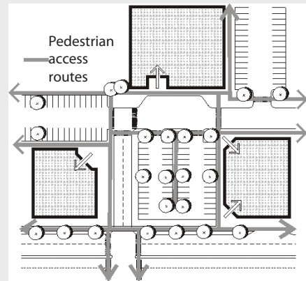
Figure 5-31. An example of an integrated pedestrian circulation system. Note the connections from the street, between buildings, through parking lots, and to adjacent sites.
