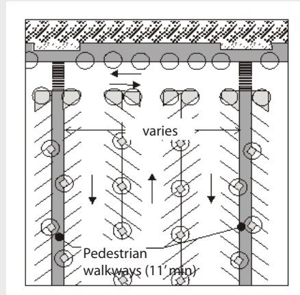
Figure 5-32. An example of a parking lot design that includes pedestrian routes.
