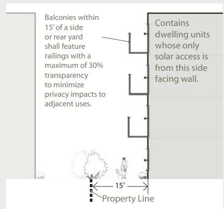
Figure 5-11. Illustrating special solar access setback requirements along the side and rear yard.
