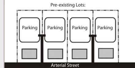
Figure 5-47. Acceptable multi-driveway example: Shared driveways between adjacent parcels.
