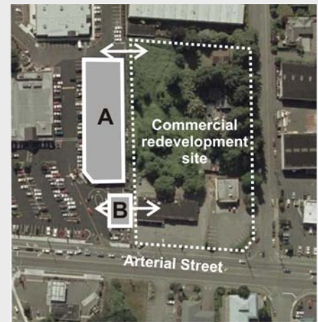
Figure 5-43. Current on-site conditions. The configuration of existing Buildings A and B make vehicular and pedestrian connectivity a challenge, but there are some opportunities.
