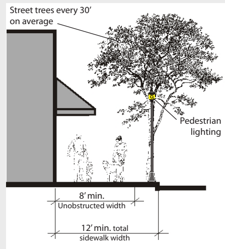
Figure 5-34. Minimum internal walkway requirements along the facade of mixed-use and retail buildings 100 feet or more in width
