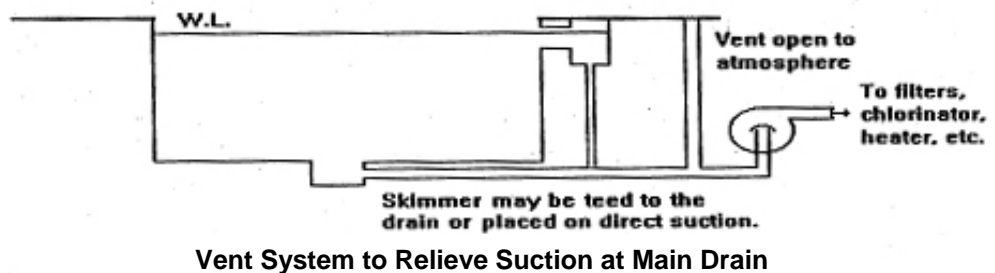
Figure 5b. Vent System to Relieve Suction at Main Drain.
