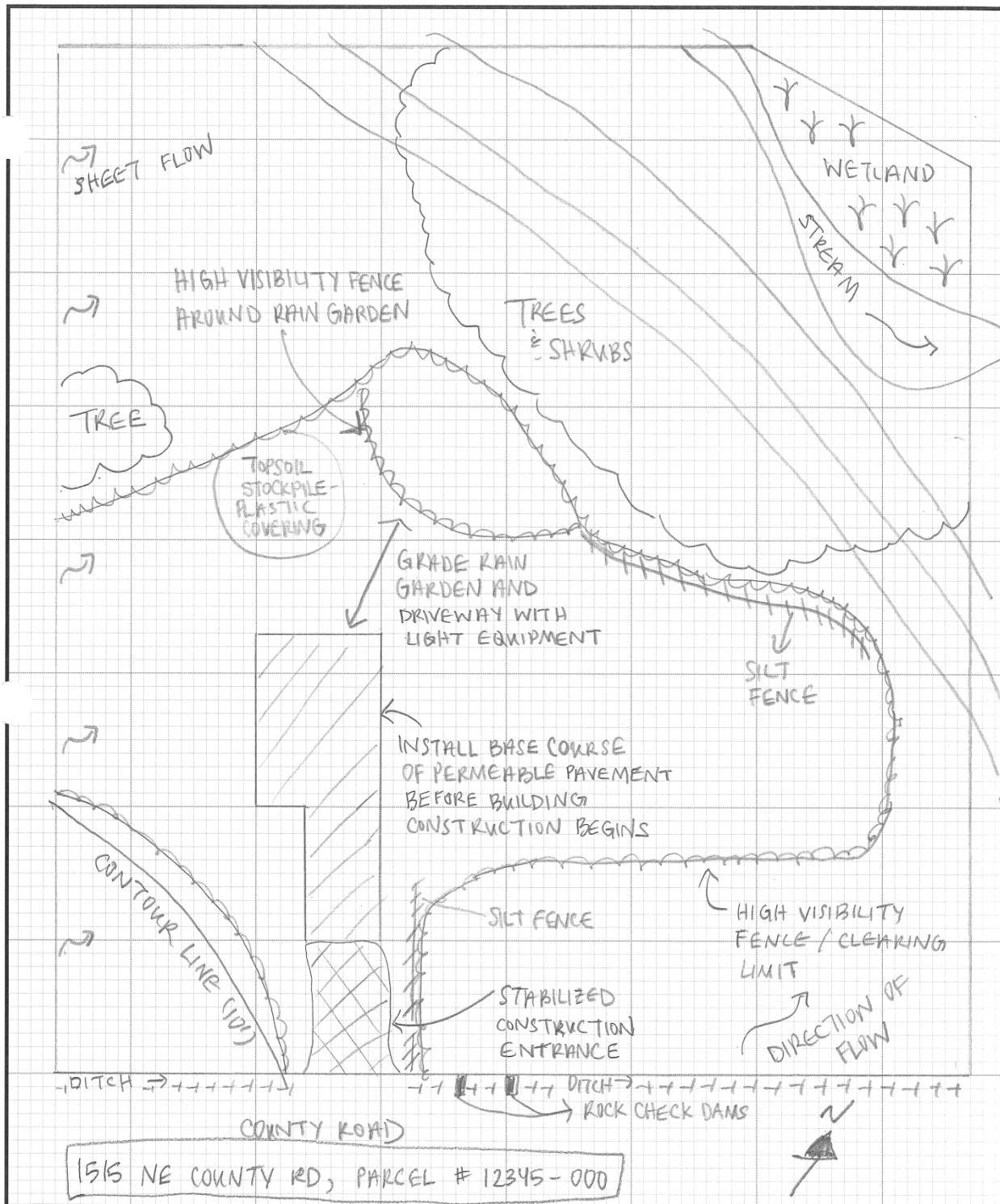
Figure 1: Example Sediment and Erosion Control Site Plan
