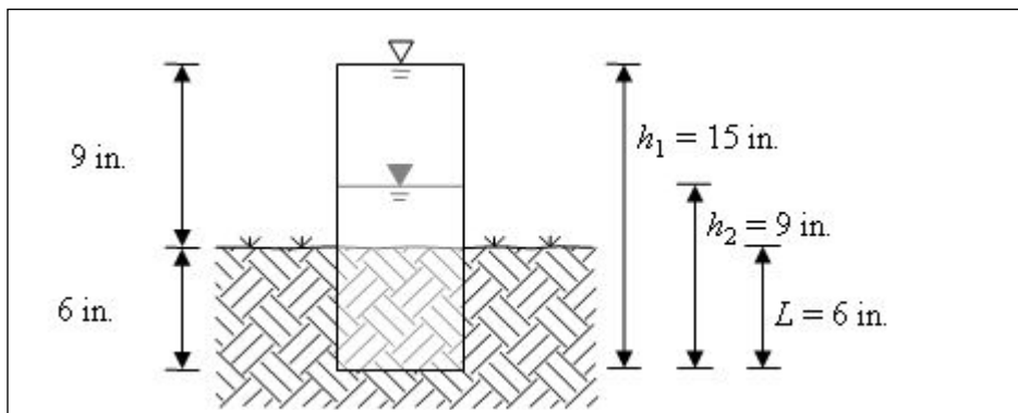
■ FIGURE 6-1. Single-Ring Falling Head Infiltration Test Procedure
