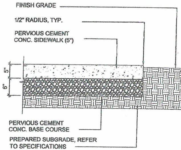
A PERVIOUS CEMENT CONC. SIDEWALK (5") SCALE: 1"=1'-0"
